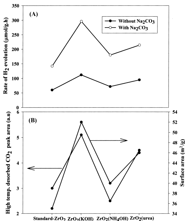
Fig. 5. Correlations among the high temperature \text{CO}_2 desorption peak areas, surface areas, and rates of \text{H}_2 evolution with and without \text{Na}_2\text{CO}_3 .
